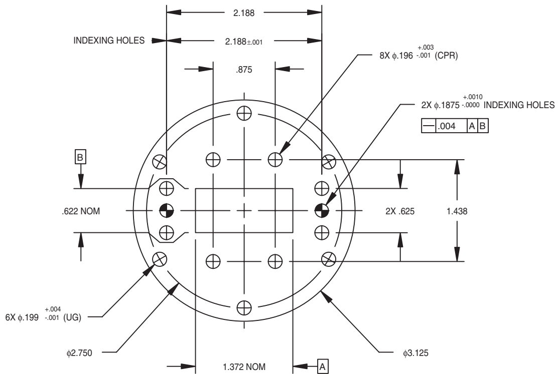
Figure 1: MPF137 Flange Interface with Critical Dimensions
