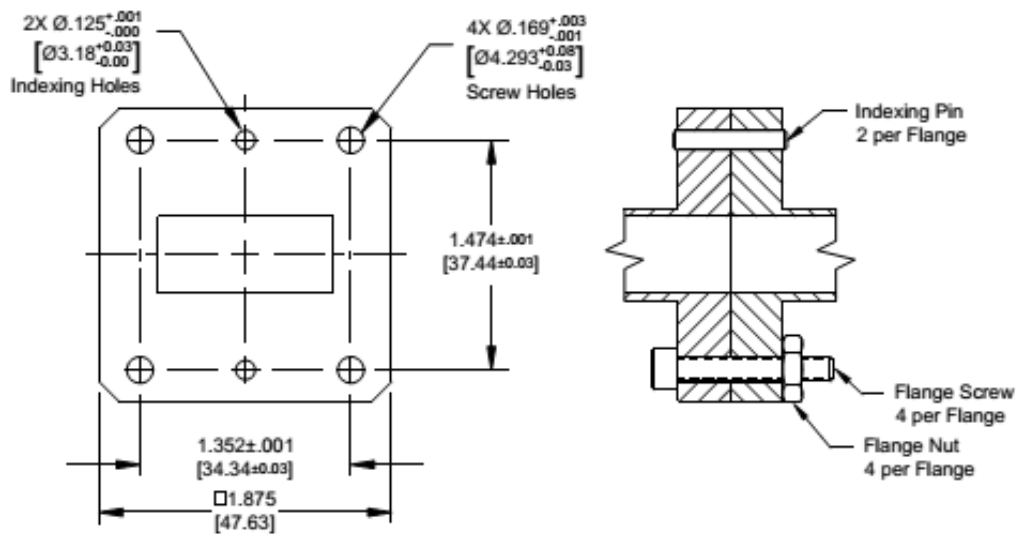
Figure 1. Flange with Indexing Pins
