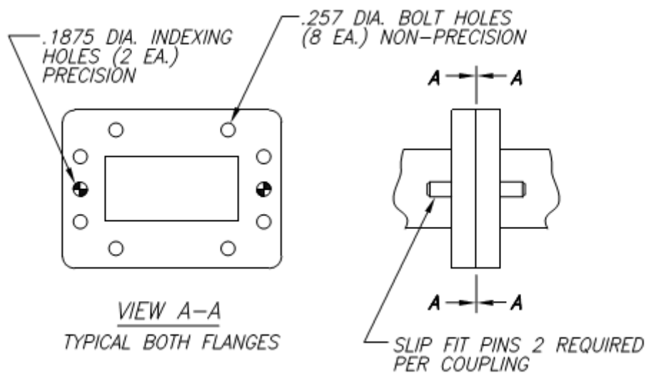
Figure 1. Flange with Indexing Pins
