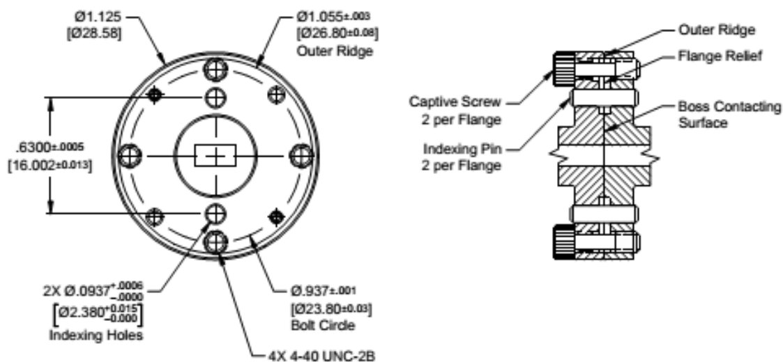
Figure 1. Flange with Indexing Pins
