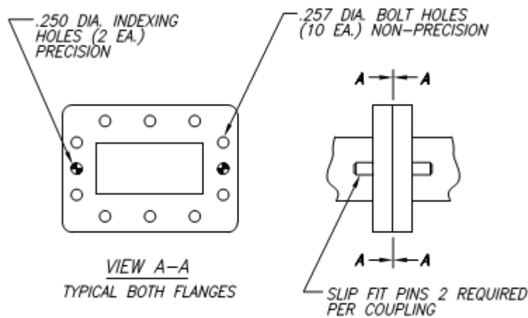
Figure 1. Flange with Indexing Pins
