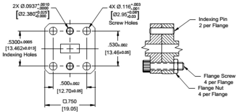
Figure 1. Flange with Indexing Pins
