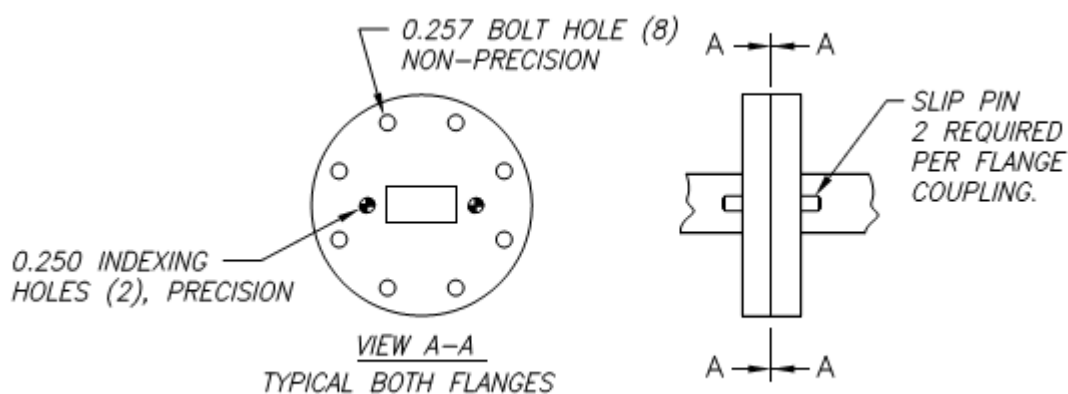
Figure 1. Flange with Indexing Pins
