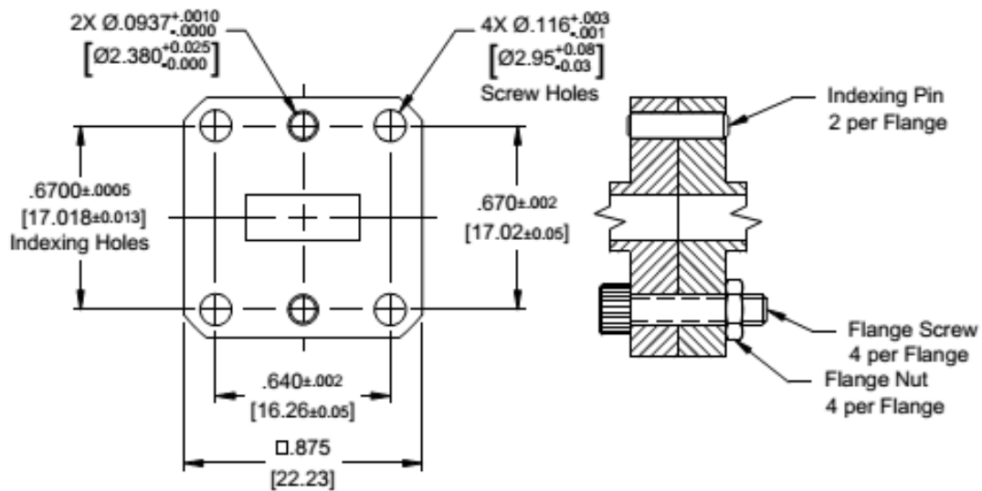
Figure 1. Flange with Indexing Pins
