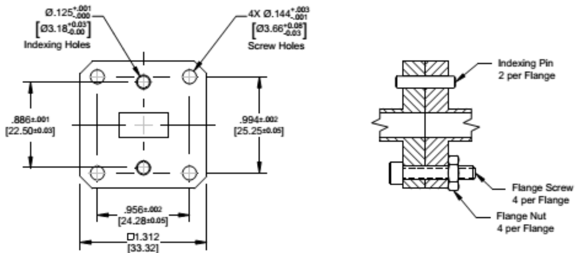
Figure 1. Flange with Indexing Pins
