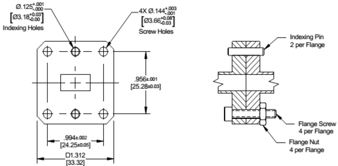
Figure 1. Flange with Indexing Pins
