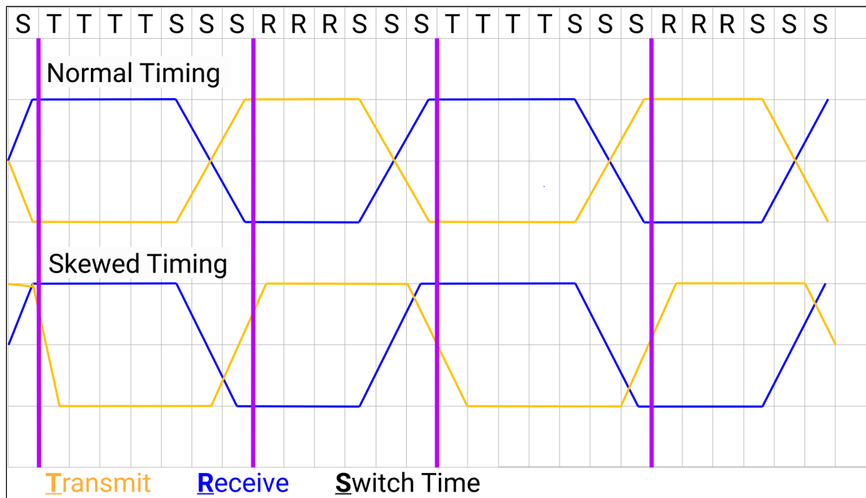
Figure 2: Ideal timing of TDD switches exhibit extreme precision, with handoffs occurring uniformly within the delay frames between transmit (yellow) and receive (blue) operations. Skewed timing caused by propagation delay, for example, can lead to switching overlap and leading data errors, among other challenges, which decreases the integrity of TDD transmissions.
