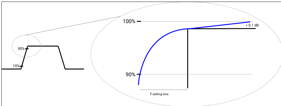
Figure 1: Magnified view of pulse vertical settling time. Settling time of a signal (90% to < 0.1 dB of its maximum value). Response Time = Rise Time + Settling Time
