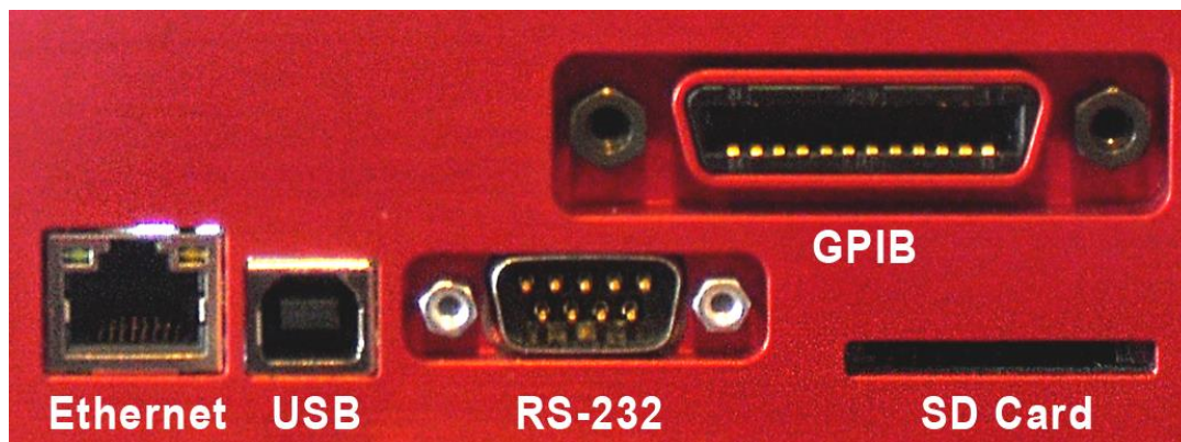
HSX Series Communication Ports
