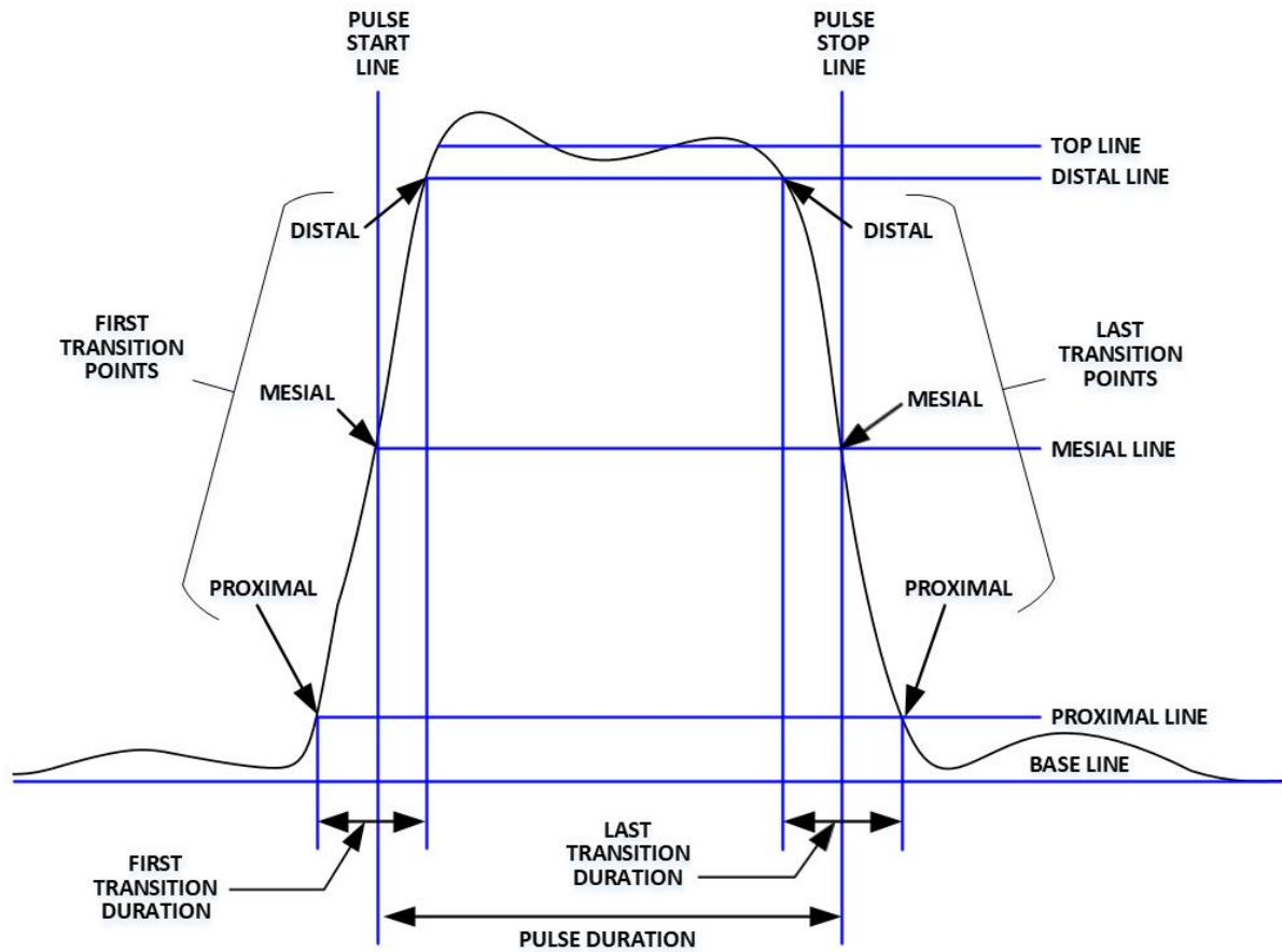
Figure 5-4. IEEE Standard Pulse (IEEE Std 194™-1977)
