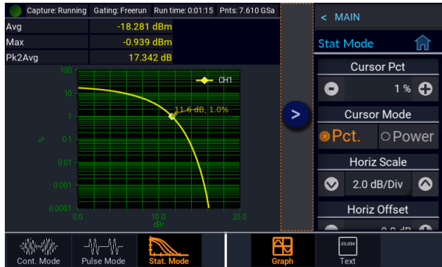
Figure 3-8. CCDF Plot With Menu Showing Cursor at 1%
