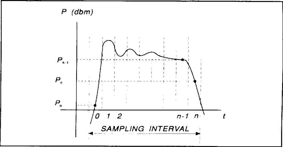
Figure 5-7. Sampling Intervals
