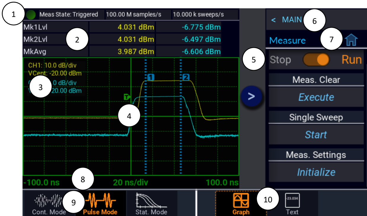
Figure 3-3. PMX40 Graph Display Using Pulse Measure Mode With Menus Exposed
