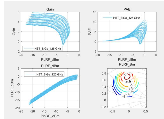
Gain vs power out (top left), power-added efficiency vs power out (top right), power out vs power for each gamma load in (bottom left), and power out contour (bottom right)
