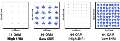
Effect of AWGN on 16-QAM and 64-QAM constellations.
