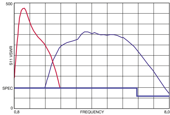
VSWR versus Frequency for XT981HL13 automated tuners.
