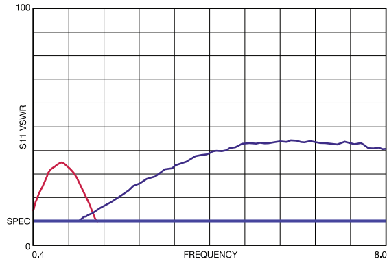
VSWR versus Frequency for XT981BL18 automated tuners.
