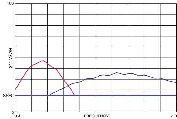
VSWR versus Frequency for XT981BL10 automated tuners.
