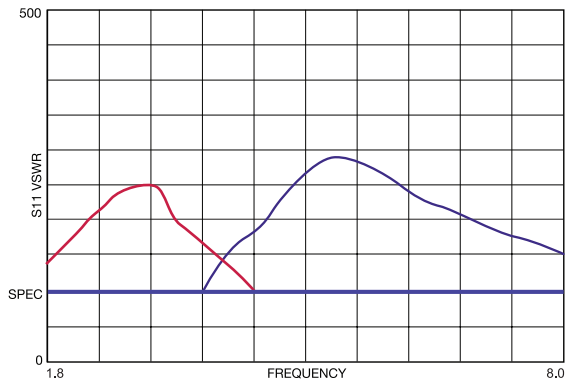
VSWR versus Frequency for XT981HL14 automated tuners.
