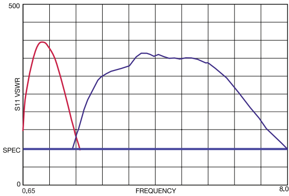
VSWR versus Frequency for XT981HL16 automated tuners.
