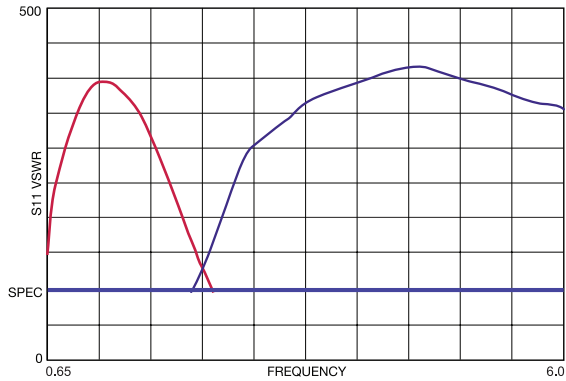
VSWR versus Frequency for XT981HL15 automated tuners.
