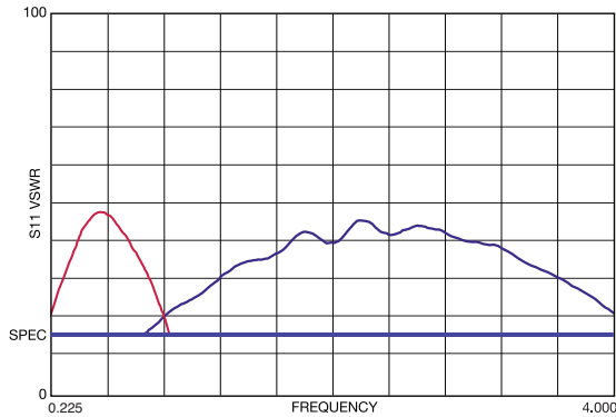
VSWR versus Frequency for XT981AL14 automated tuners.
