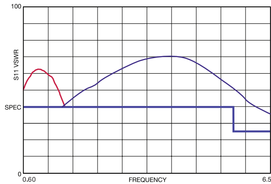
VSWR versus Frequency for XT981VL10 automated tuners.
