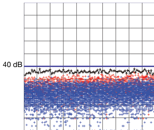
S11 Repeatability
