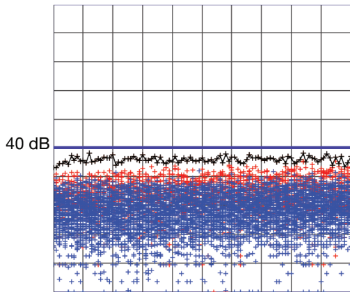
S11 Repeatability
