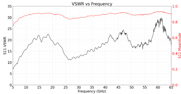
VSWR versus Frequency for NT-8G-65G-1C automated tuners.
