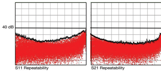
Repeatability for NT-8G-65G-1C-C automated tuners.
