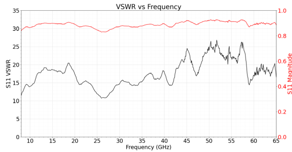
VSWR versus Frequency for NT-8G-65G-1C-C automated tuners.
