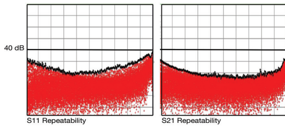
Repeatability for NT-18G-50G-1C-C automated tuners.
