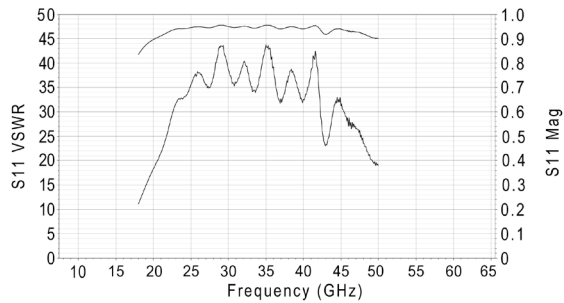
VSWR versus Frequency for NT-18G-50G-1C automated tuners.
