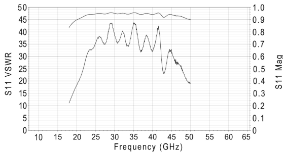
VSWR versus Frequency for NT-18G-50G-1C-C automated tuners.
