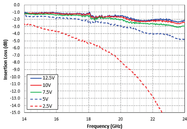
Figure 11a: HX5100-1424 Insertion Loss
